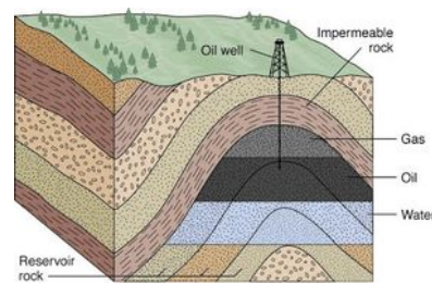
Figure 8.5: Oil and gas embedded in porous rock, under an impermeable caprock [42]. From U. Calgary.
