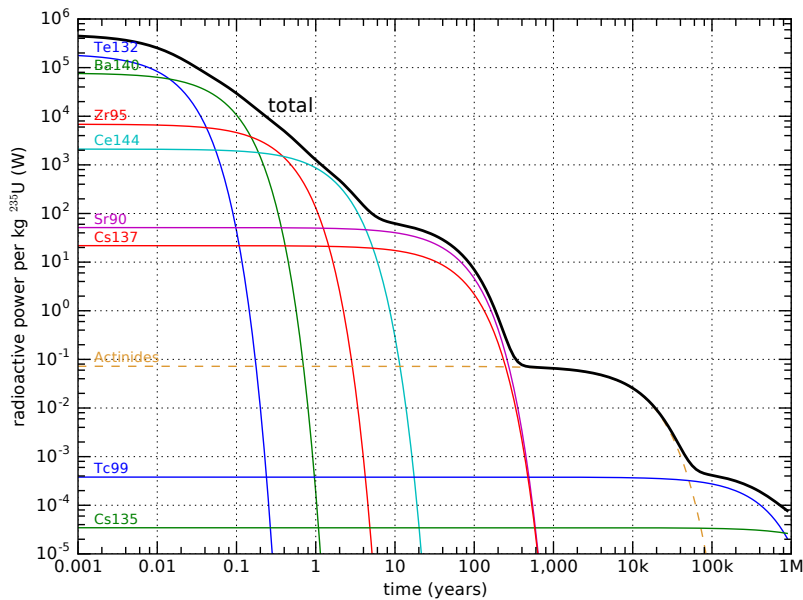
Figure 15.19: Decay activity of fragments from 1 kg of fissioned ^{235}\text{U} over time, on a log–log plot. The vertical axis is the power of radioactive emission, in W, for a variety of relevant isotopes—each having their own characteristic half life. The black line at the top is the total activity (sum of all contributions), and some of the key individuals are separated out. The dashed line for actinides is an approximate representative indicator of the role played by heavy nuclides formed in the reactor by uranium absorption of neutrons. Minor tick marks are at multipliers of 2, 4, 6, and 8 for each axis. As a matter of possible interest, the exponential decays of each element on this log–log plot have the functional form of exponential curves drawn upside-down.
