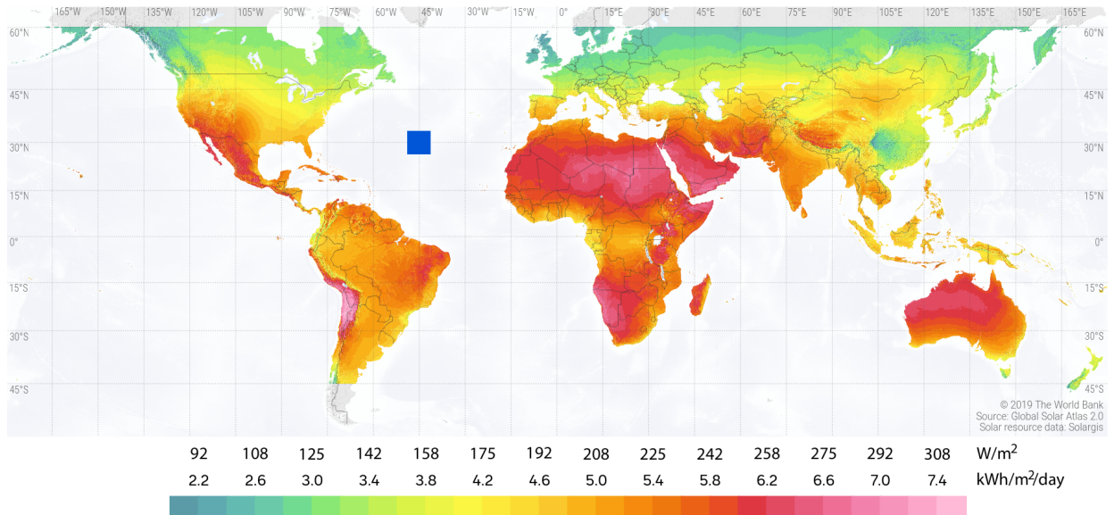
Figure 13.8: Insolation onto locally horizontal surfaces for the world (for flat plates facing directly upward), in units of \text{W/m}^2 and \text{kWh/m}^2/\text{day} . The area of the blue square in the middle of the Atlantic ocean is enough to satisfy current global energy demand, using 15% efficient solar collection (but distributed, of course). Source: The World Bank.
