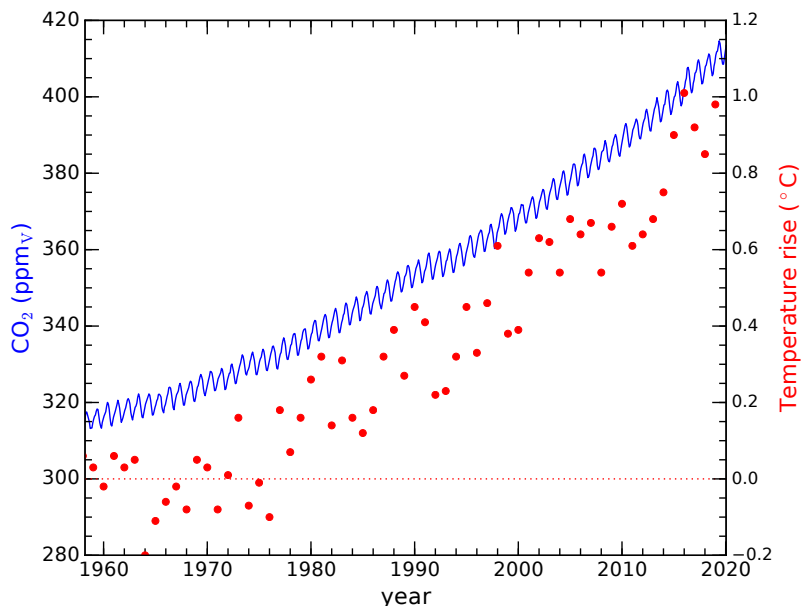
Figure 9.1: In blue (left axis), CO 2 measurements from Mauna Loa (Hawaii) for the last 60 years, showing a relentless and accelerating upward trend now at about 2.6 ppm v per year [50]. Seasonal variations due to photosynthesis are seen on top of this trend. Pre-industrial levels were around 280 ppm v , so that we have added about 130 parts per million (ppm). Red dots (right axis) show global average mean temperature records over the same period [51]. Thus far, global average temperature has risen about 1°C. Note that the Kyoto Protocol in 1997 and Paris Agreement in 2015 (Box 19.4; p. 320) do not visibly curb the upward trajectory of CO 2 emissions.
